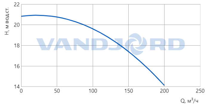
— NBV 125-250-11/4 Q-A-D-E-B-A-E
