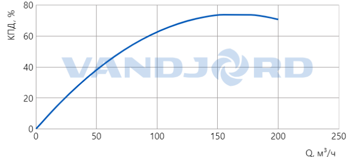
— NBV 125-250-11/4 Q-A-D-E-B-A-E
