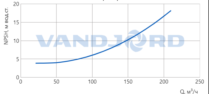
VNK 125-100/200 Q-A-E-B-AB-E
