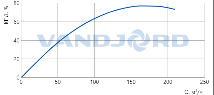
VNK 125-100/200 Q-A-E-B-AB-E
