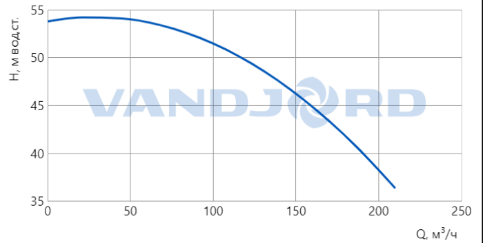
VNK 125-100/200 Q-A-E-B-AB-E
